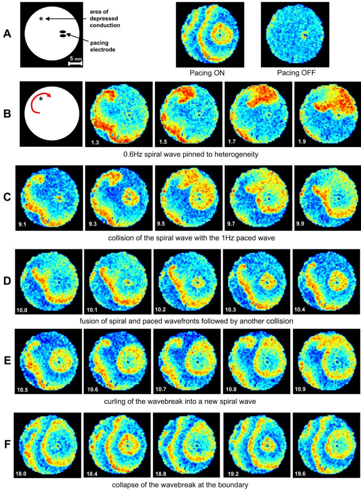
Fig. 7. Paced-induced spiral wave detachment and subsequent termination due to wave break collision with a boundary. A : location of pacing electrodes and a local heterogeneity ( left ) and circular wave fronts of paced waves (note changes in wave curvature near local heterogeneity) and appearance of the cell layer after overdrive pacing was turned off ( right ). B : 4 sequential frames showing spiral wave pinned to a heterogeneity. C : 5 sequential frames showing collision of the spiral wave with the paced wave. D : 5 sequential frames showing the 2 waves coalescing into a single wave front. E : 5 sequential frames showing curling of the wave break into a new spiral wave. F : 5 sequential frames showing collapse of the wave break at the boundary. Time (in seconds) is shown in each frame.
