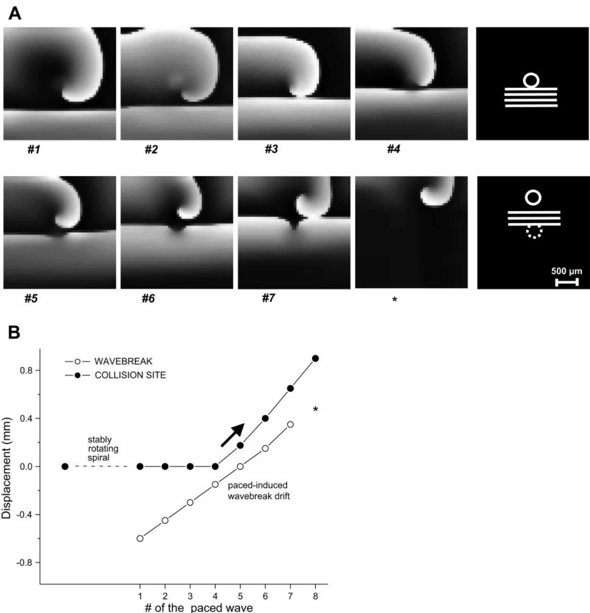
Fig. 6. Paced-induced drift of spiral wave: numerical study. A : impending collisions between the spiral wave and 4 consecutive paced waves before they reach the tip ( top row ) and 3 impending collisions of the spiral wave and paced waves during paced-induced drift ( bottom row ). Right : relative positions of collision site (white lines) and wave break (solid circle). Dotted circle, area of local heterogeneity similar to that in Fig. 4 D . B : graphical illustration of the process in A . ○, Position of the wave break; ●, collision site coordinates. *, Illustration that the wavebreak displacement occurs as a result of the previous collision (paced wave 7), and not due to the collision with what will be the next paced wave (wave 8).
