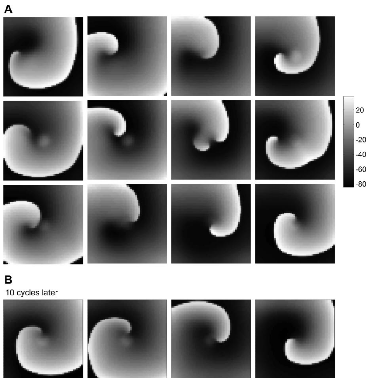
Fig. 3. Capture of a nearby spiral by a local heterogeneity. A : 12 sequential frames show how a small area of heterogeneity, seen as a slightly brighter spot at the center, attracts the tip of a spiral wave. B : 4 sequential frames 10 cycles after the capture event shown in A . They illustrate that spiral remained stable and pinned to the same spot. Full sequence can be seen in the online supplement 1 .
