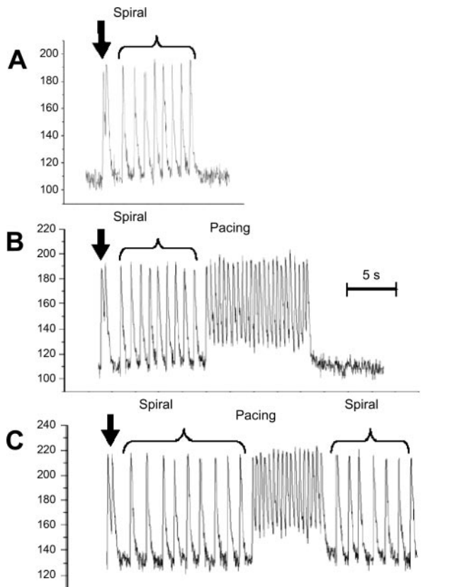
Fig. 1. Three types of behavior observed for induced reentrant (spiral) activity. Recordings of Ca 2+ transients are shown as relative units of fluo 4 fluorescence. Arrows indicate the application of premature stimuli, which initiated a reentrant wave. A: self-termination of a reentrant wave. B: reentrant wave termination by overdrive pacing. C: unsuccessful termination of reentrant wave activation by overdrive pacing.
