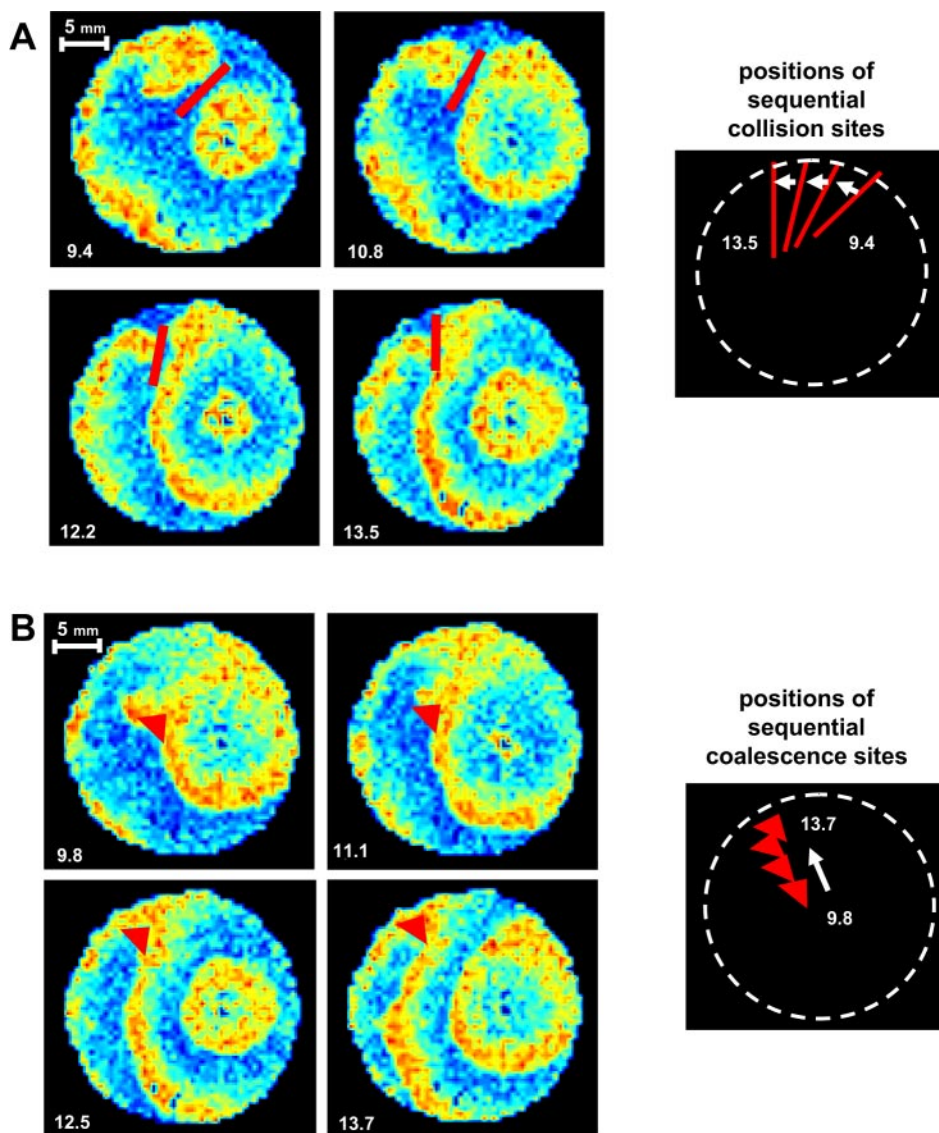
Fig. 8. Paced-induced movements of collision and coalescence sites. A : sequential frames illustrate movement of the collision site (red bar). B : sequential frames illustrate movement of a point where the 2 waves coalesce (red triangle). Corresponding cartoons are shown at right . Time (in seconds) is shown in each frame.
