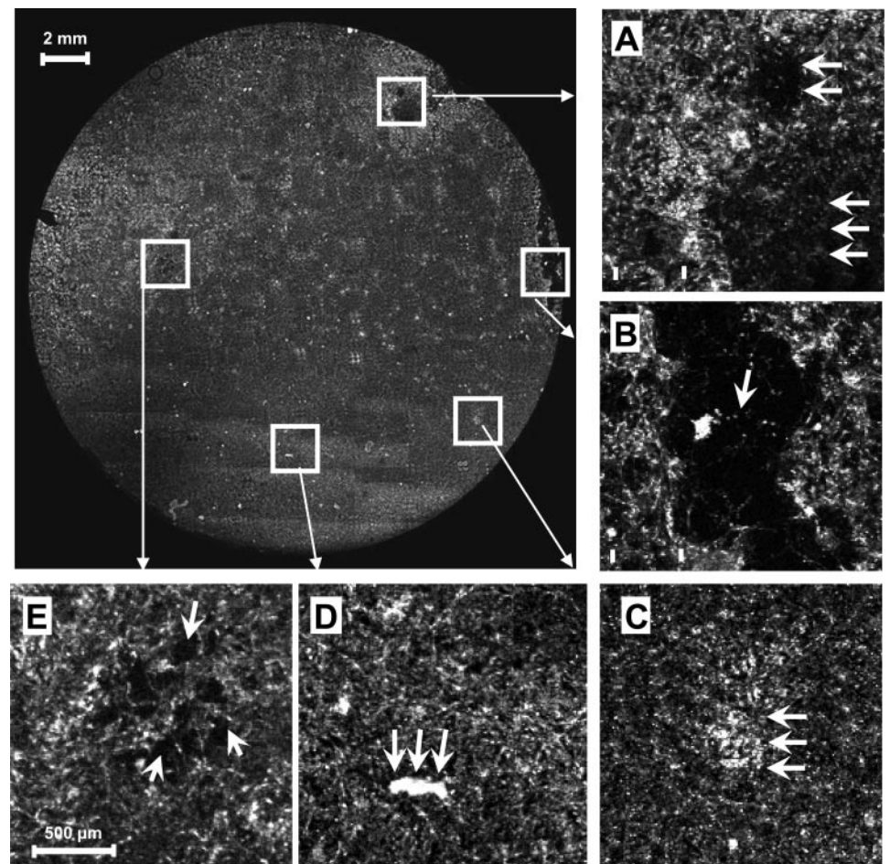
Fig. 2. Endogenous heterogeneities in macroscopically homogenous coverslips. A : myocyte-free regions; B : mechanical damage due to forceps during coverslip transfer; C : areas of higher density; D : clusters of damaged cells on top of the monolayer (arrows); E : areas of lesser/uneven density.
