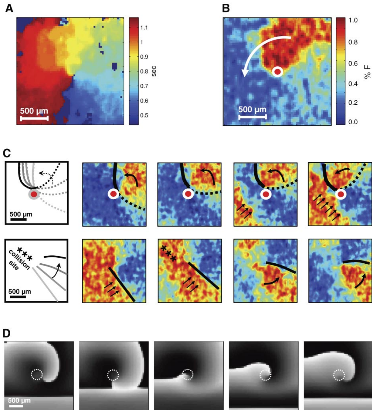
Fig. 4. Reentrant wave terminated by rapid pacing. A : 1 complete rotation of the reentrant wave presented as an activation map, where color indicates time of activation at each pixel. B : fluorescence snapshot of the wave. Arrow denotes direction of rotation. Normalized fluo 4 fluorescence is shown in pseudocolor. Red dot indicates position of the spiral tip. C : sequence of frames illustrating interaction of 1 paced wave front with the tip of the spiral wave before ( top row ) and after ( bottom row ) collision. Last 2 frames show formation of a wave break. ***, Site of collision. Solid lines, wave fronts; dotted lines, wave backs. Red dot indicates position of the spiral tip. D : numerical illustration of the process described in C . Dotted circle, position of a local heterogeneity [reduced time-independent K^+ current ( I_{K1} )], around which the spiral rotates.
