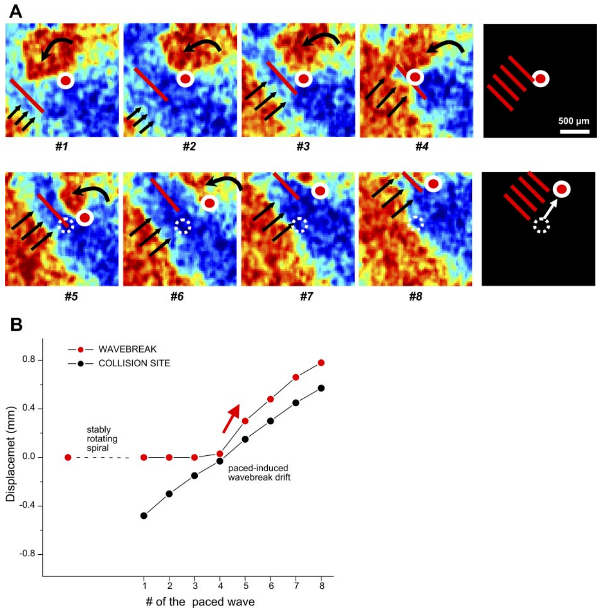
Fig. 5. Paced-induced drift of spiral waves. A : impending collisions of the spiral and 4 consecutive paced waves before they reach the tip ( top row ) and impending collisions of the spiral wave and 4 consecutive paced waves during the paced-induced drift ( bottom row ). Arrows show direction of paced wave propagation. Right : relative positions of collision site (red lines) and wave break (red circle). Dotted circle indicates location of the initial wave break; arrow shows direction of paced induced drift. At this magnification ( \sim 2 \times 2 mm area), individual cell heterogeneity is clearly visible. B : graphical illustration of process shown in A . Red dots, position of wave break; black dots, collision site coordinates. Displacement was measured in the direction of drift.
